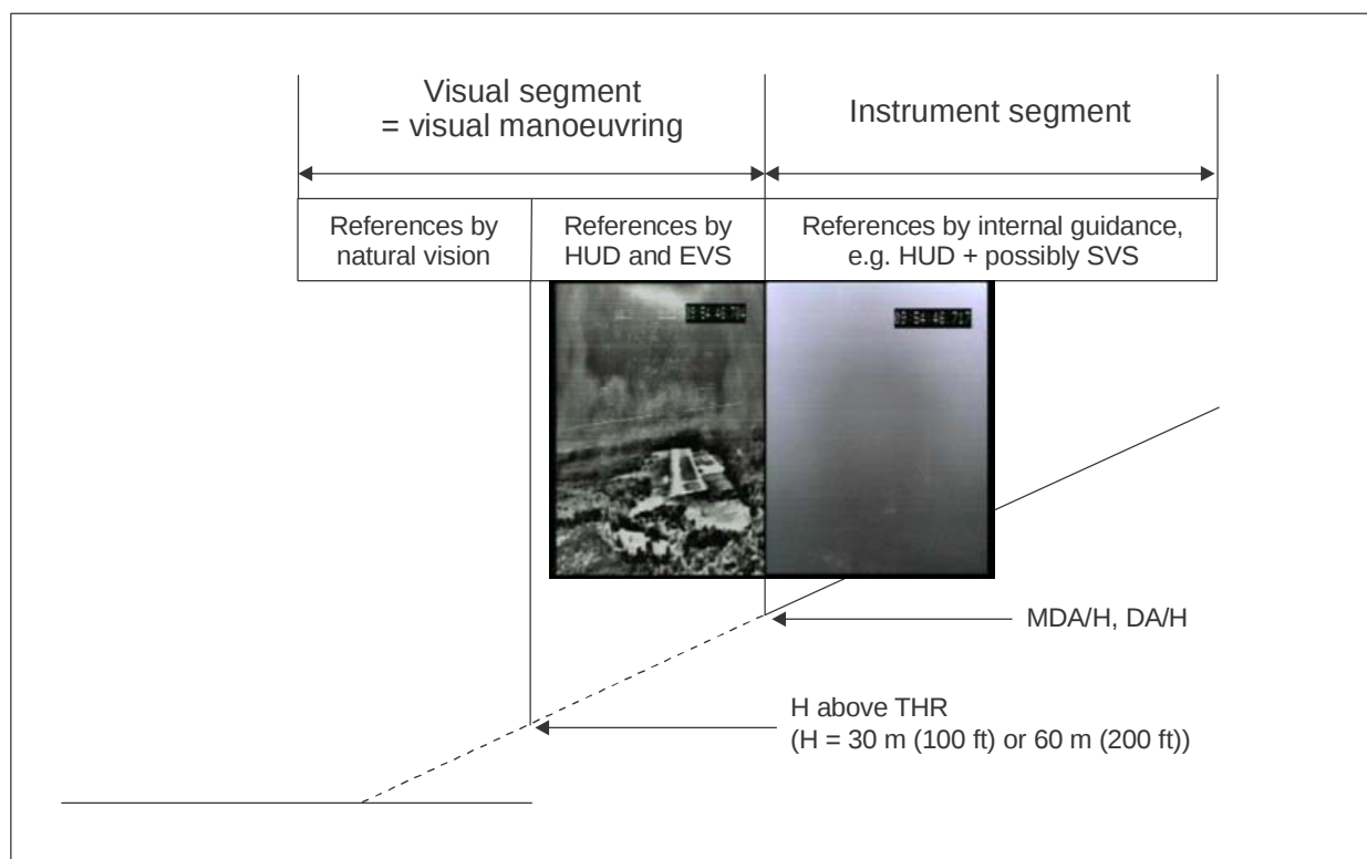
Figure H-1. EVS operations — transition from instrument to visual references
