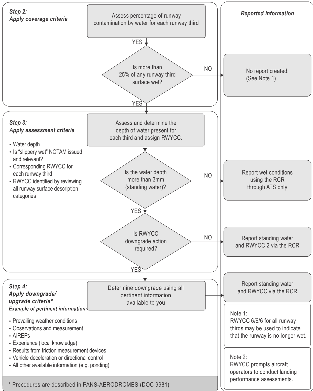
Figure 4-5. Flowchart B
